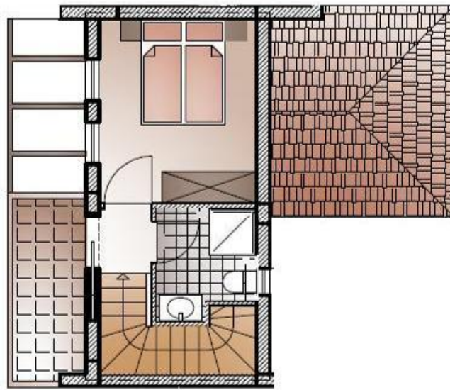
1. FLOOR
