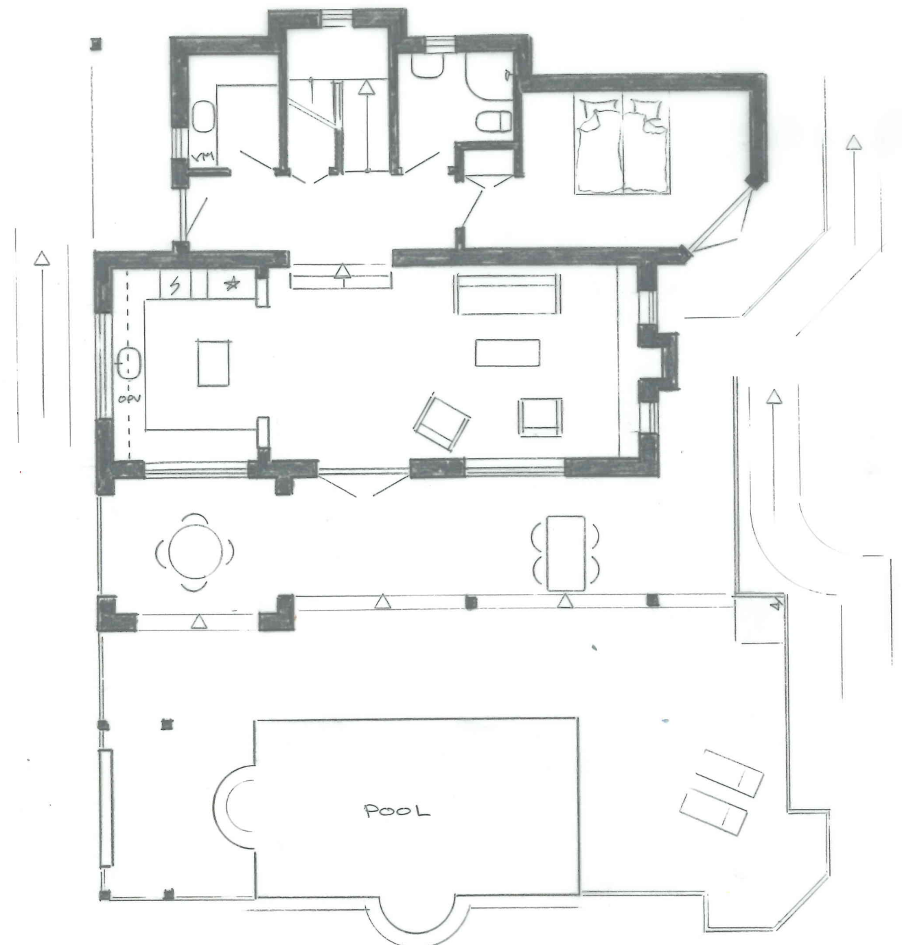
LIVING FLOOR
